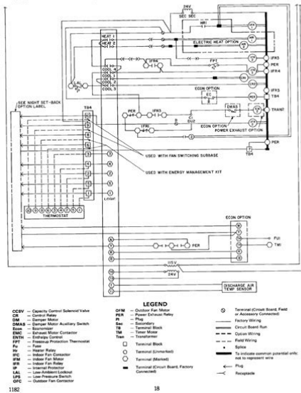
50DF Typical wiring schematic (2-speed option shown)
